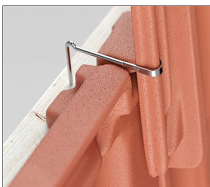
All clay and concrete roof tiles should be mechanically fixed.
